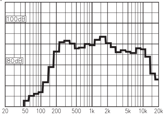
Sound pressure levels at different frequencies at 1W/1m pink noise.
