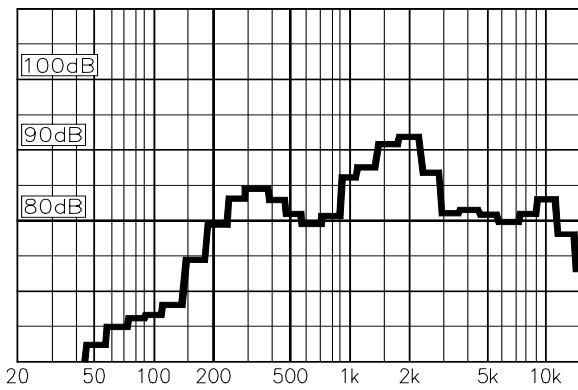
Sound pressure levels at different frequencies at 1W/1m sine wave.
