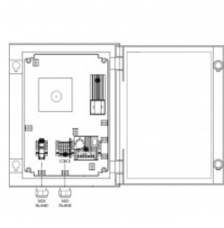
IP DECT Base Station In cabinet with heater and thermostat
