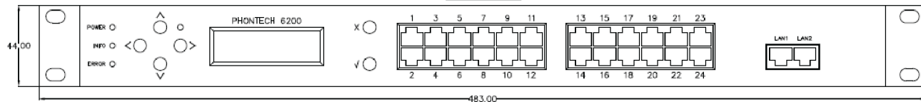
Front View
