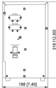
BATTERY REAR VIEW
