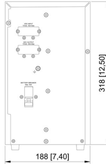
BATTERY REAR VIEW
