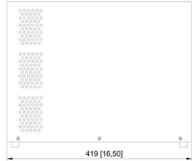
BATTERY SIDE VIEW
