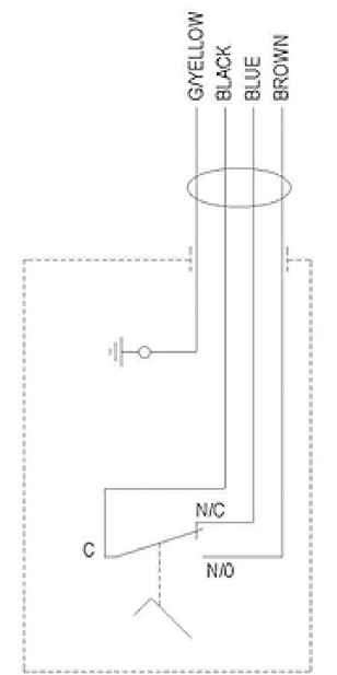
VIEWED FROM FRONT OF FOOTSWITCH
