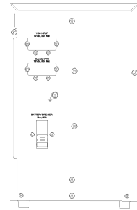
REAR VIEW
