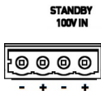
4-way pluggable Wago cage clamp (male)
