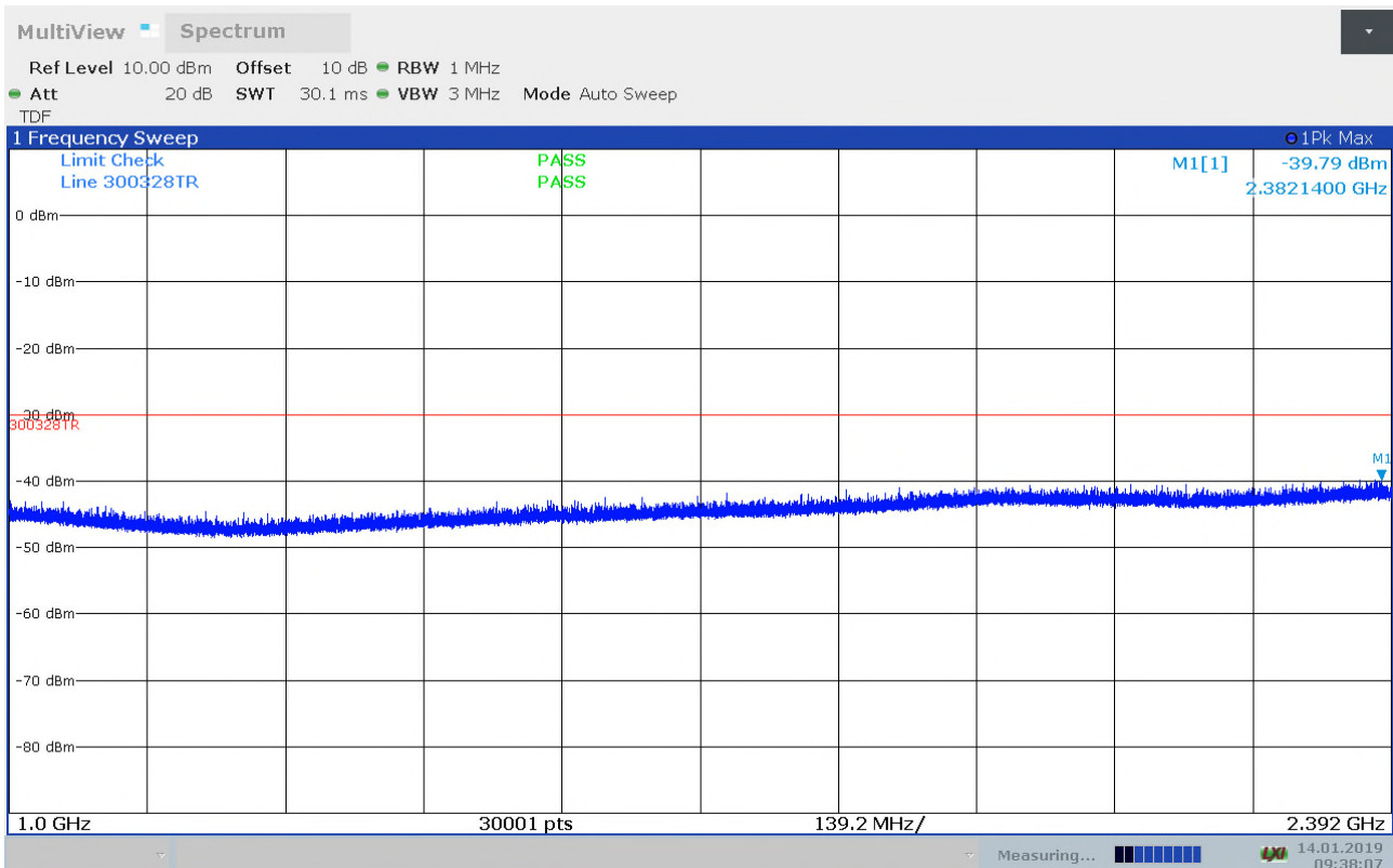
Radiated Emissions, 1 - 2.392GHz, 2412MHz, 11b, 1Mbps, VP
