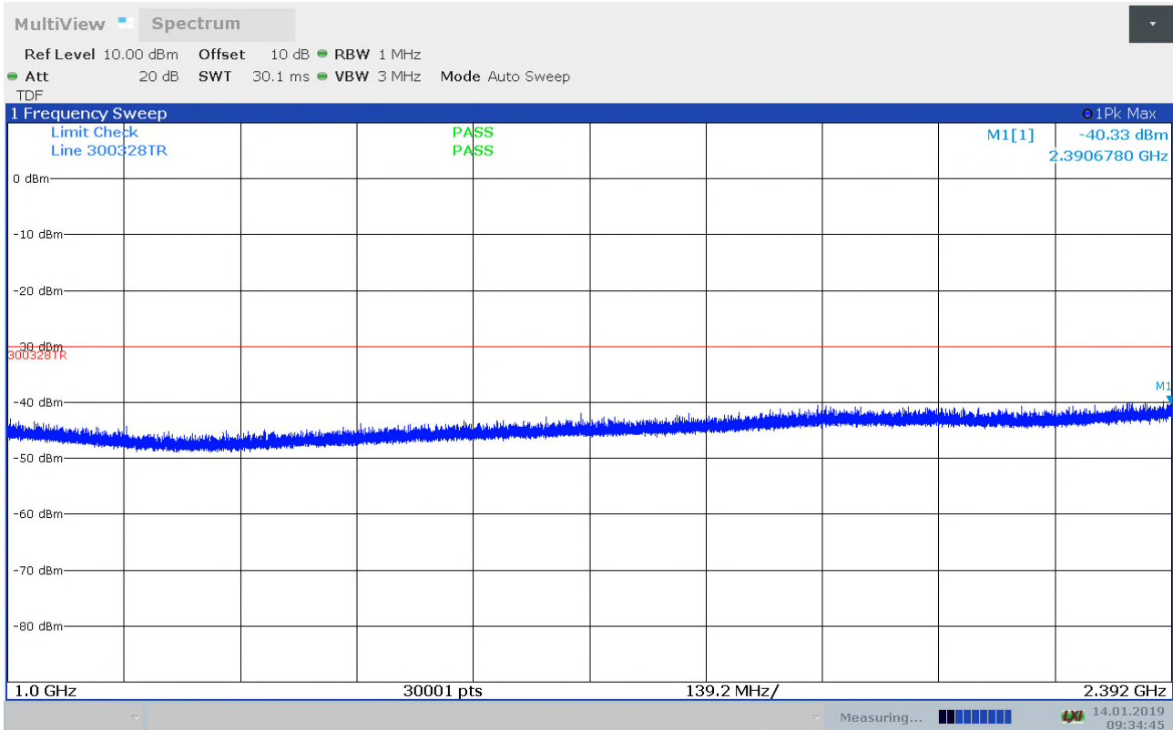
Radiated Emissions, 1 - 2.392GHz, 2412MHz, 11b, 1Mbps, HP
