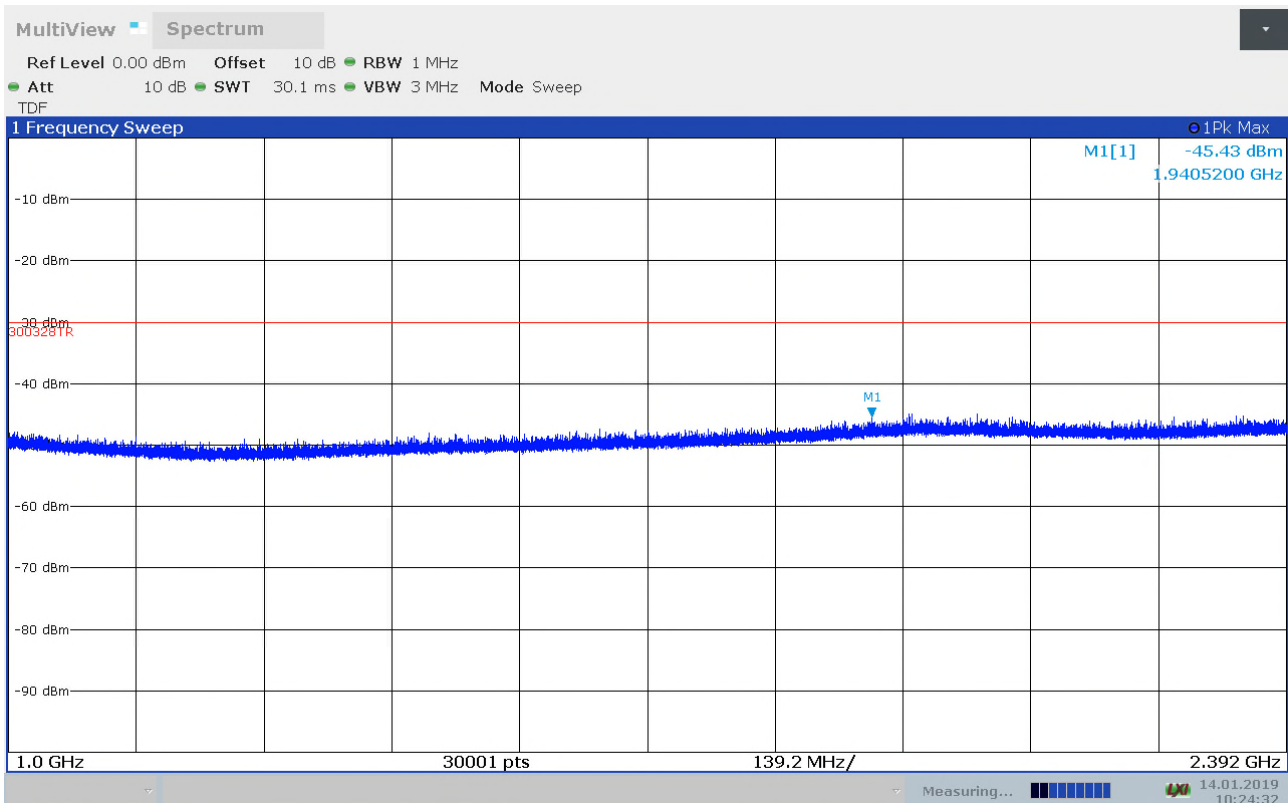
Radiated Emissions, 1 - 2.392GHz, 2472MHz, 11b, 1Mbps, VP
