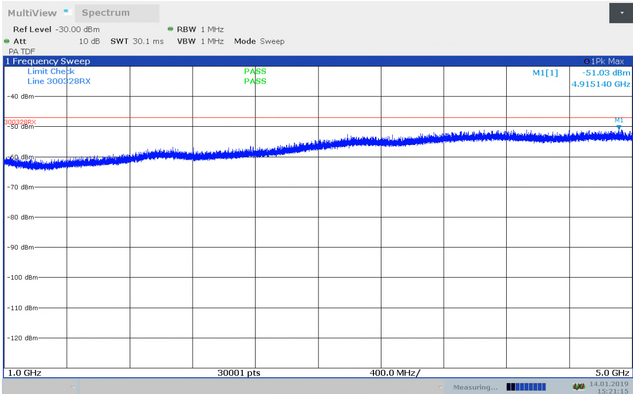
Receiver Emissions, radiated, 1 - 5GHz, ch2472MHz, HP
