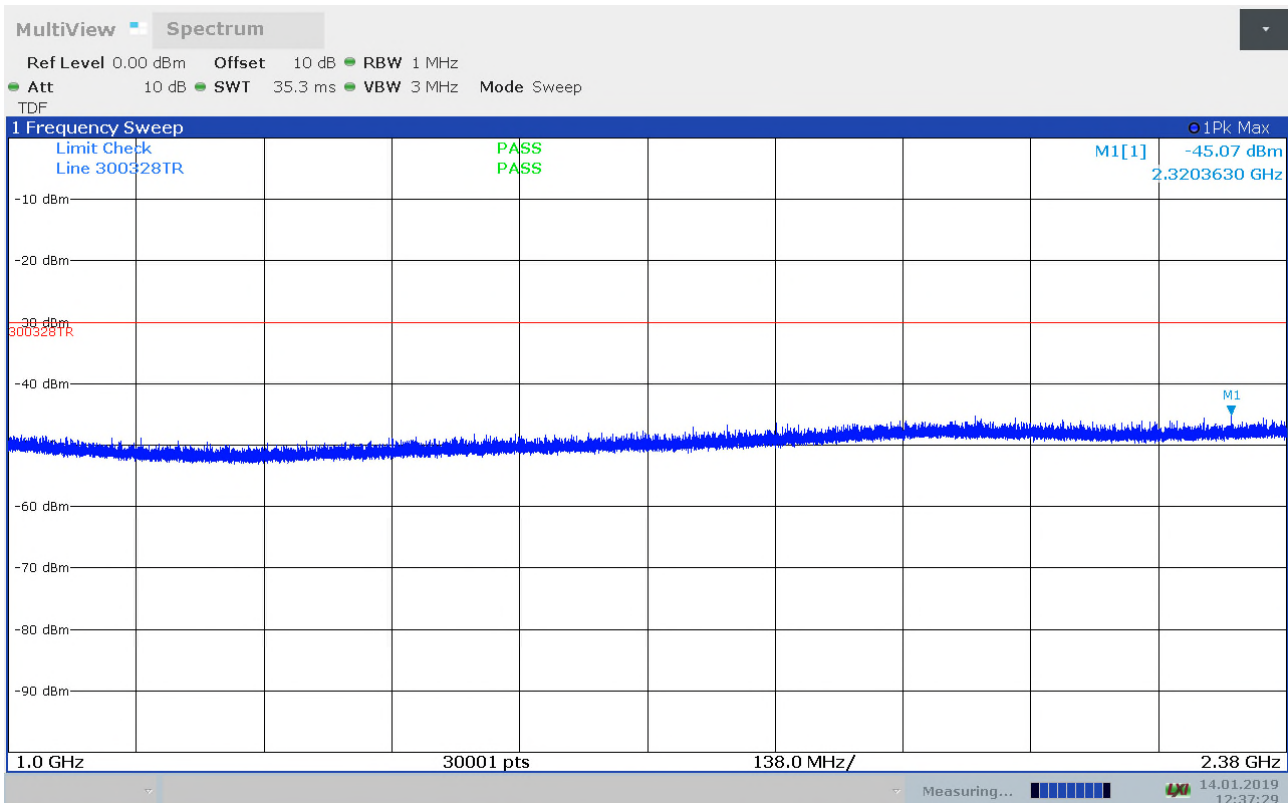
Radiated Emissions, 1 - 2.380GHz, 2472MHz, 11g, 6Mbps, VP
