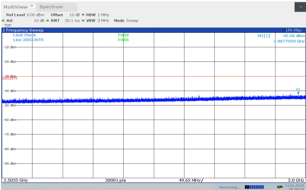
Radiated Emissions, 2.5035 - 3GHz, 2412MHz, 11g, 6Mbps, VP
