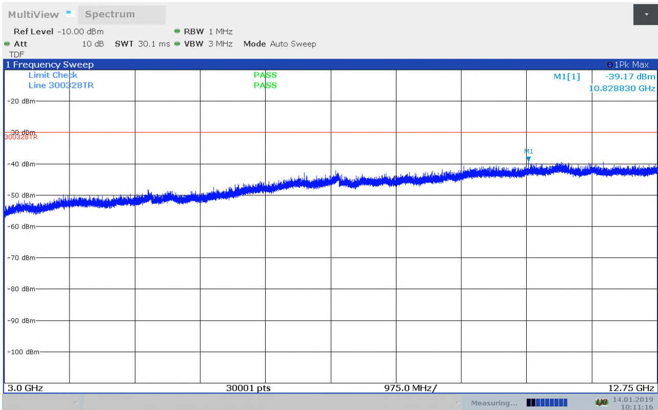
Radiated Emissions, 3 – 12.75GHz, 2472MHz, 11b,1Mbps, HP
