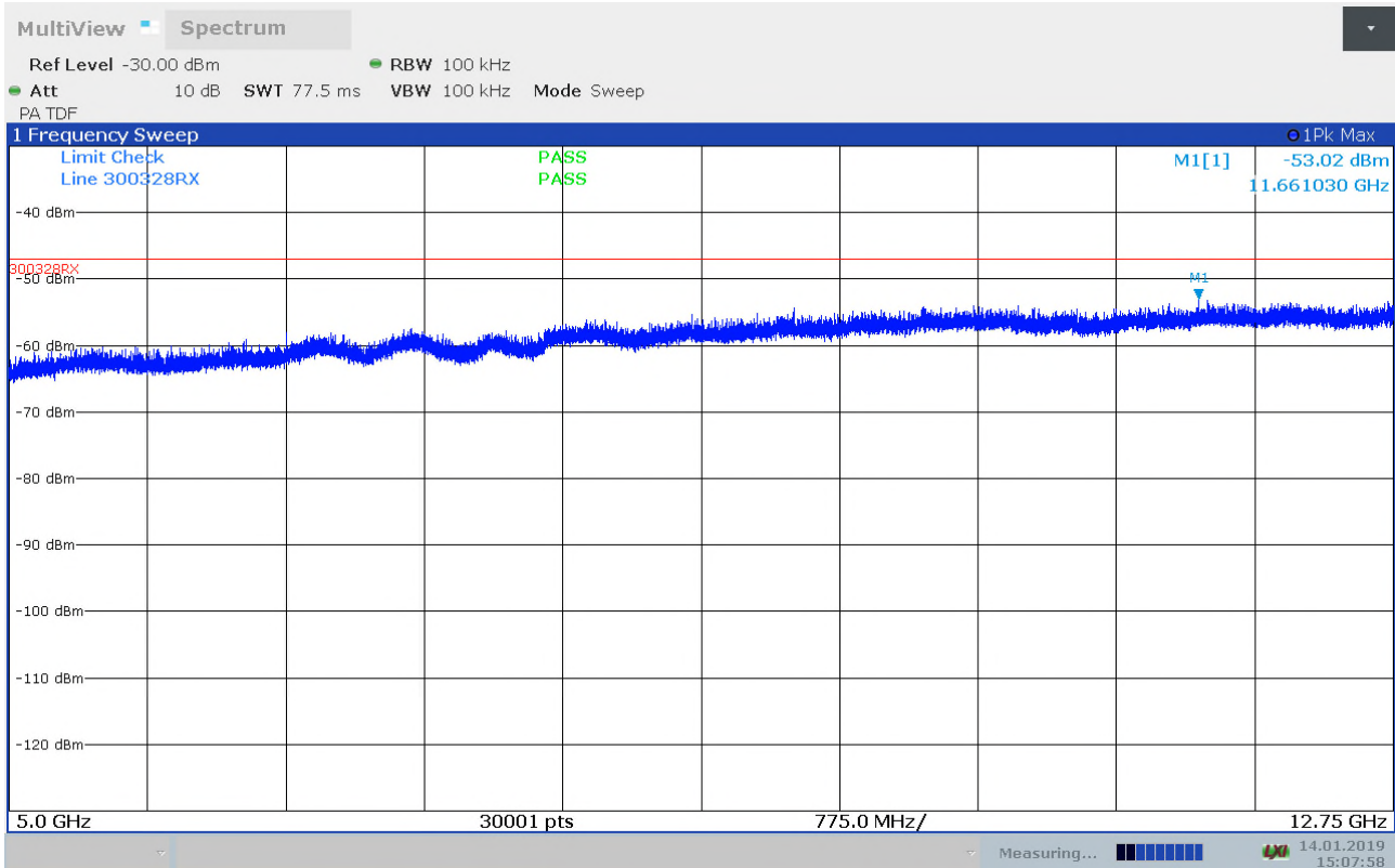
Receiver Emissions, radiated, 5 - 12.75GHz, ch2412MHz, HP, prescan
