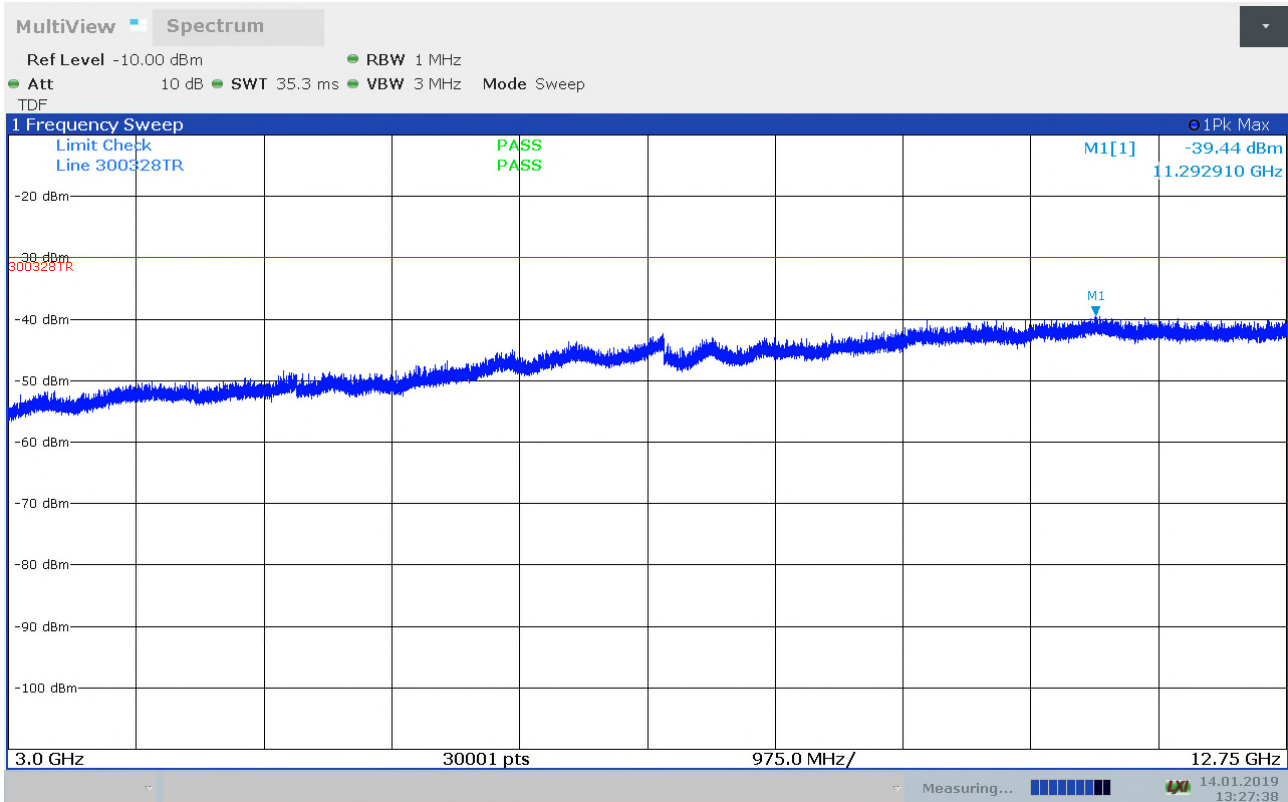
Radiated Emissions, 3 – 12.75GHz, 2472MHz, 11n, mcs0, HP
