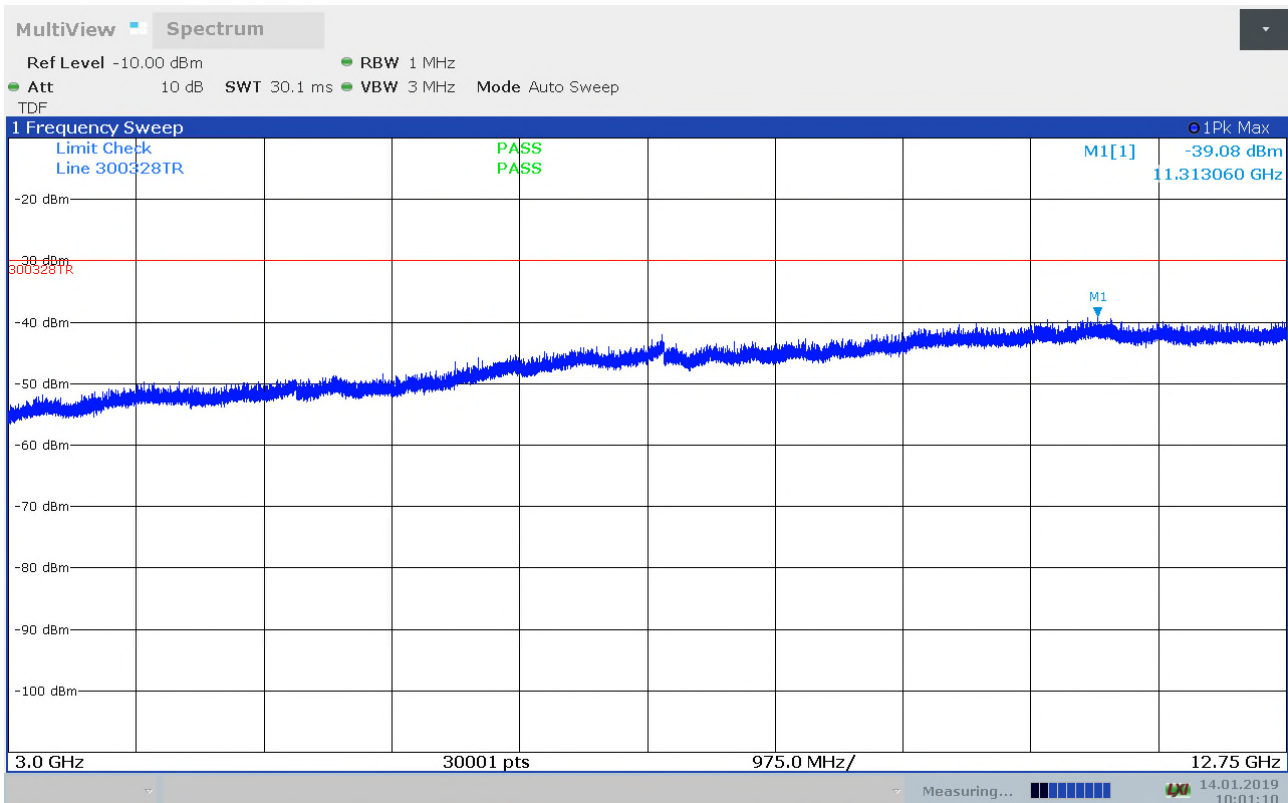
Radiated Emissions, 3 – 12.75GHz, 2412MHz, 11b, 1Mbps, VP
