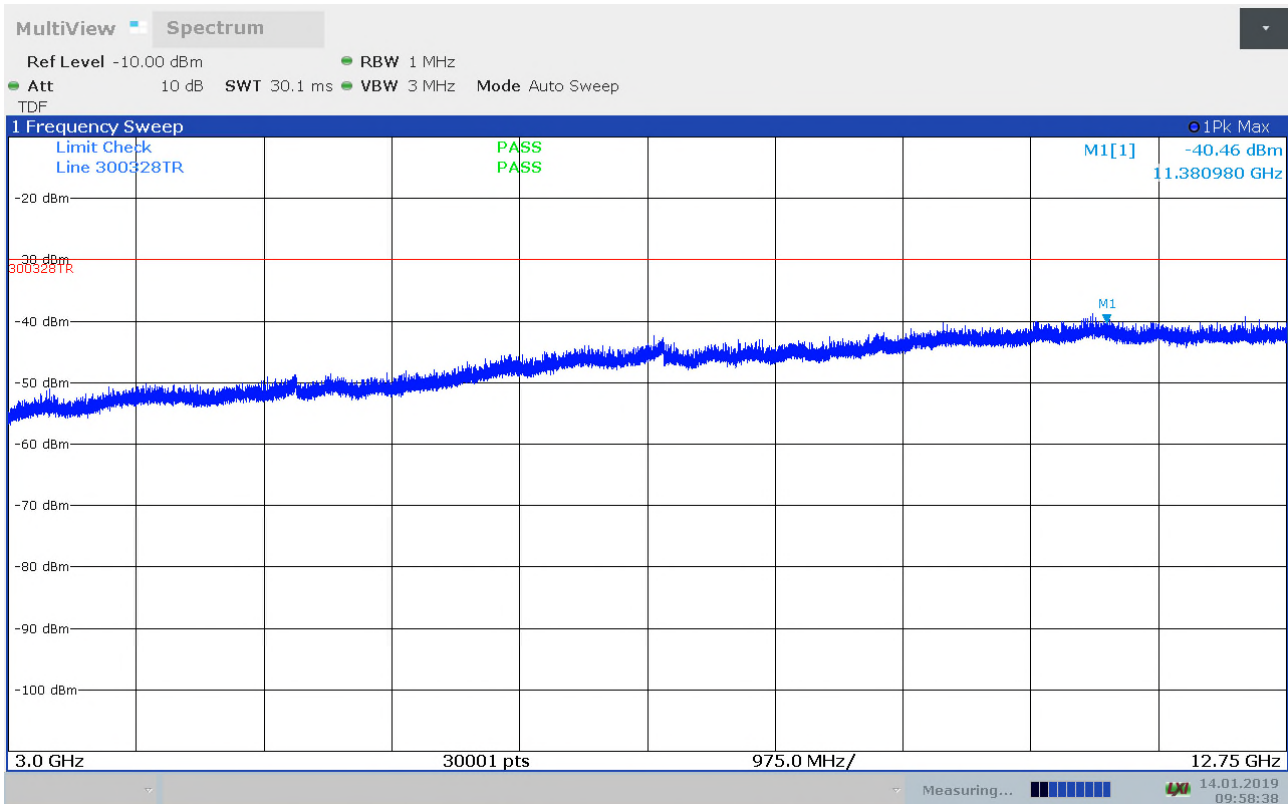
Radiated Emissions, 3 – 12.75GHz, 2412MHz, 11b, 1Mbps, HP
