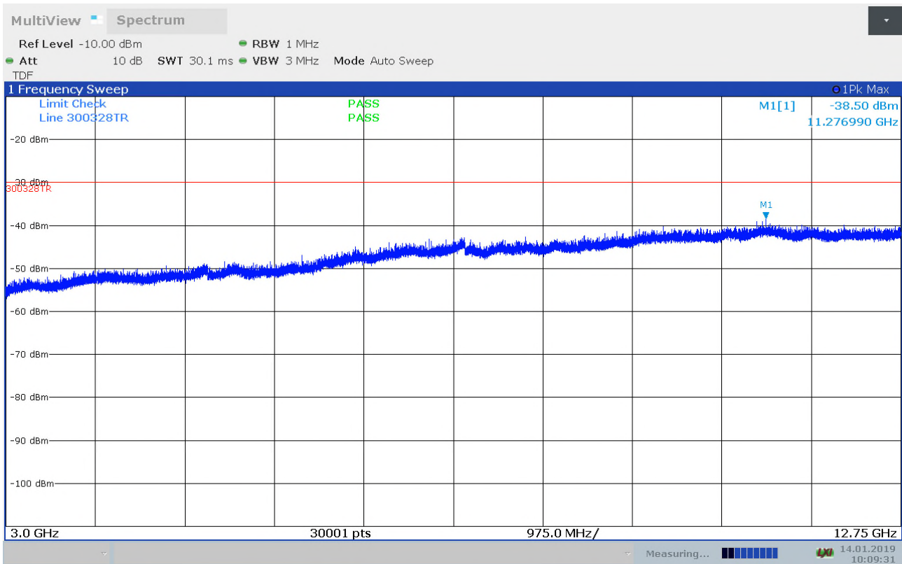
Radiated Emissions, 3 – 12.75GHz, 2472MHz, 11b,1Mbps, VP
