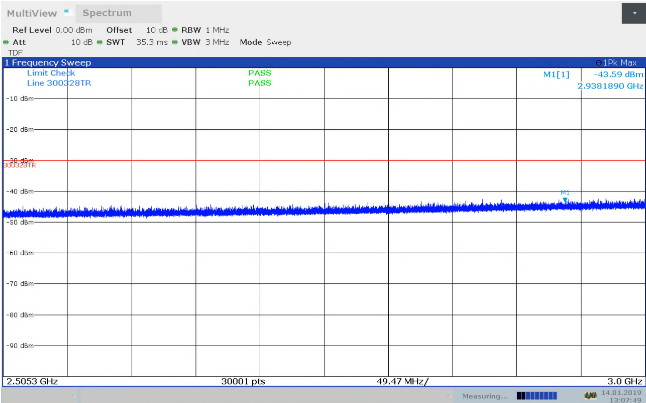
Radiated Emissions, 2.5035 - 3GHz, 2412MHz, 11n, mcs0, HP
