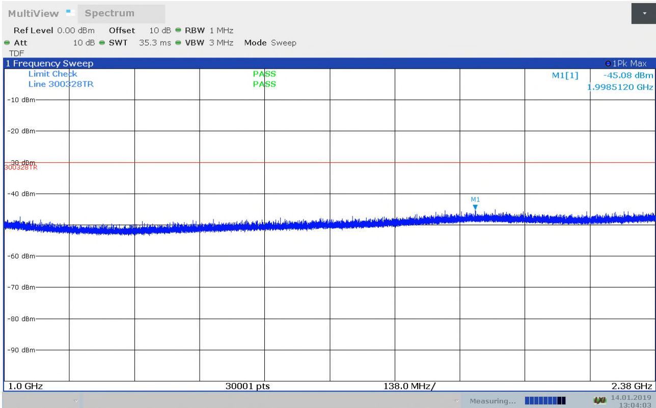
Radiated Emissions, 1 - 2.380GHz, 2412MHz, 11n, mcs0, HP
