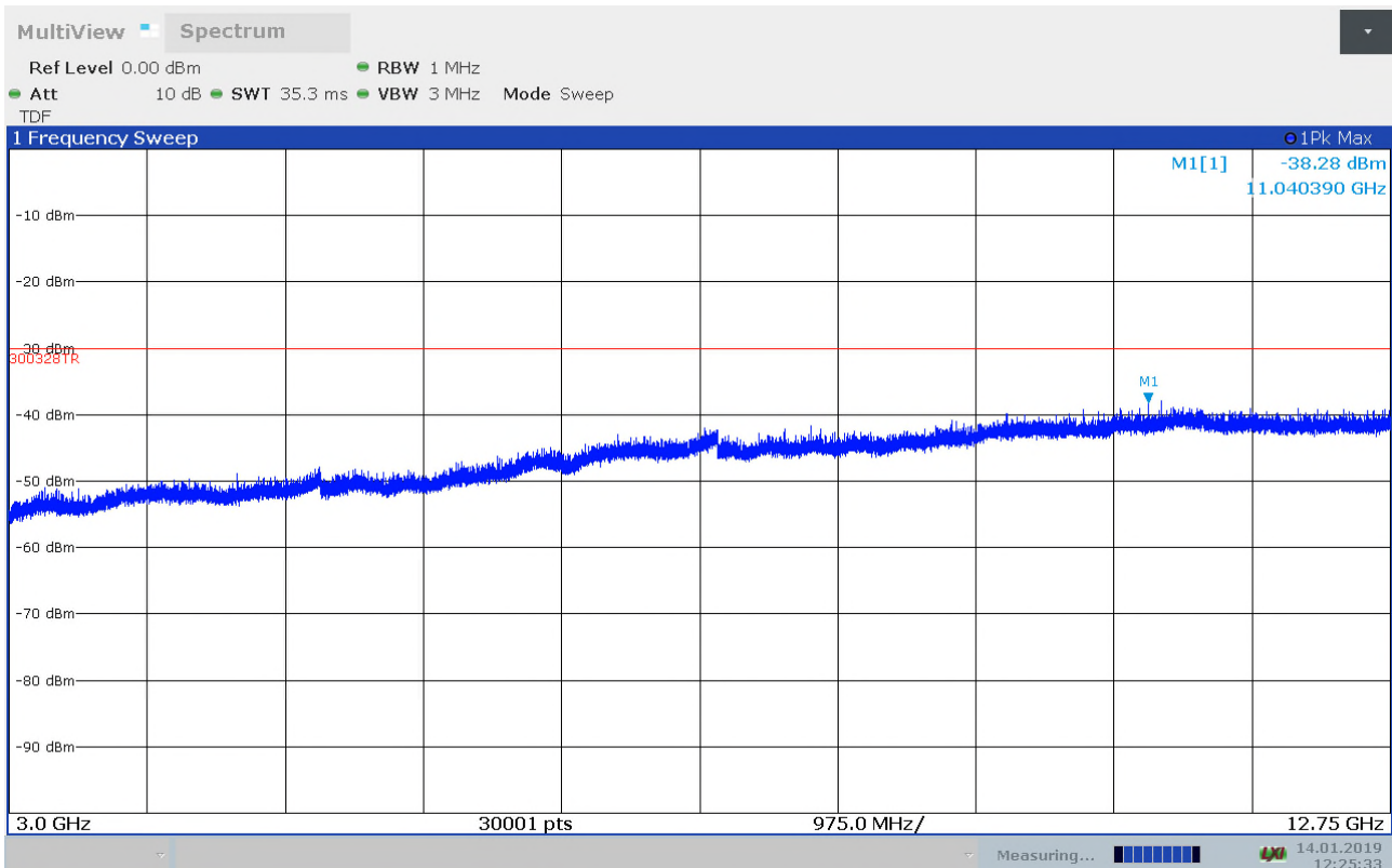
Radiated Emissions, 3 – 12.75GHz, 2472MHz, 11g,6Mbps, VP
