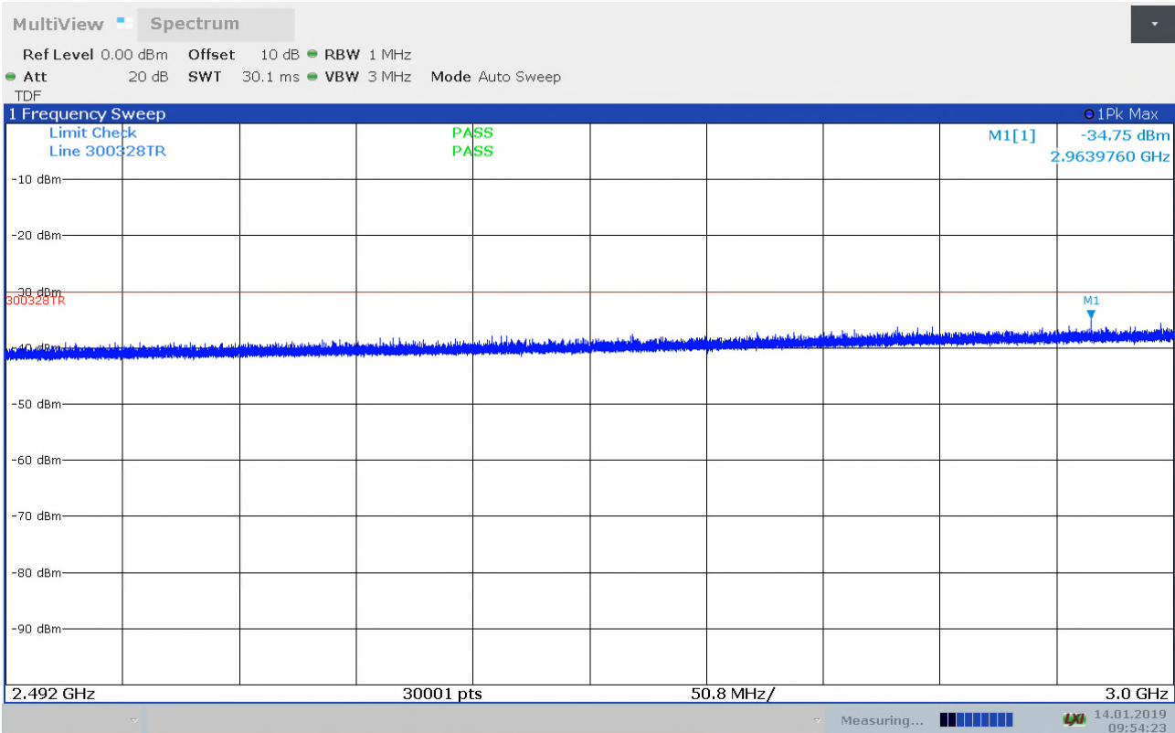
Radiated Emissions, 2.492 - 3GHz, 2412MHz,11b,1Mbps, HP
