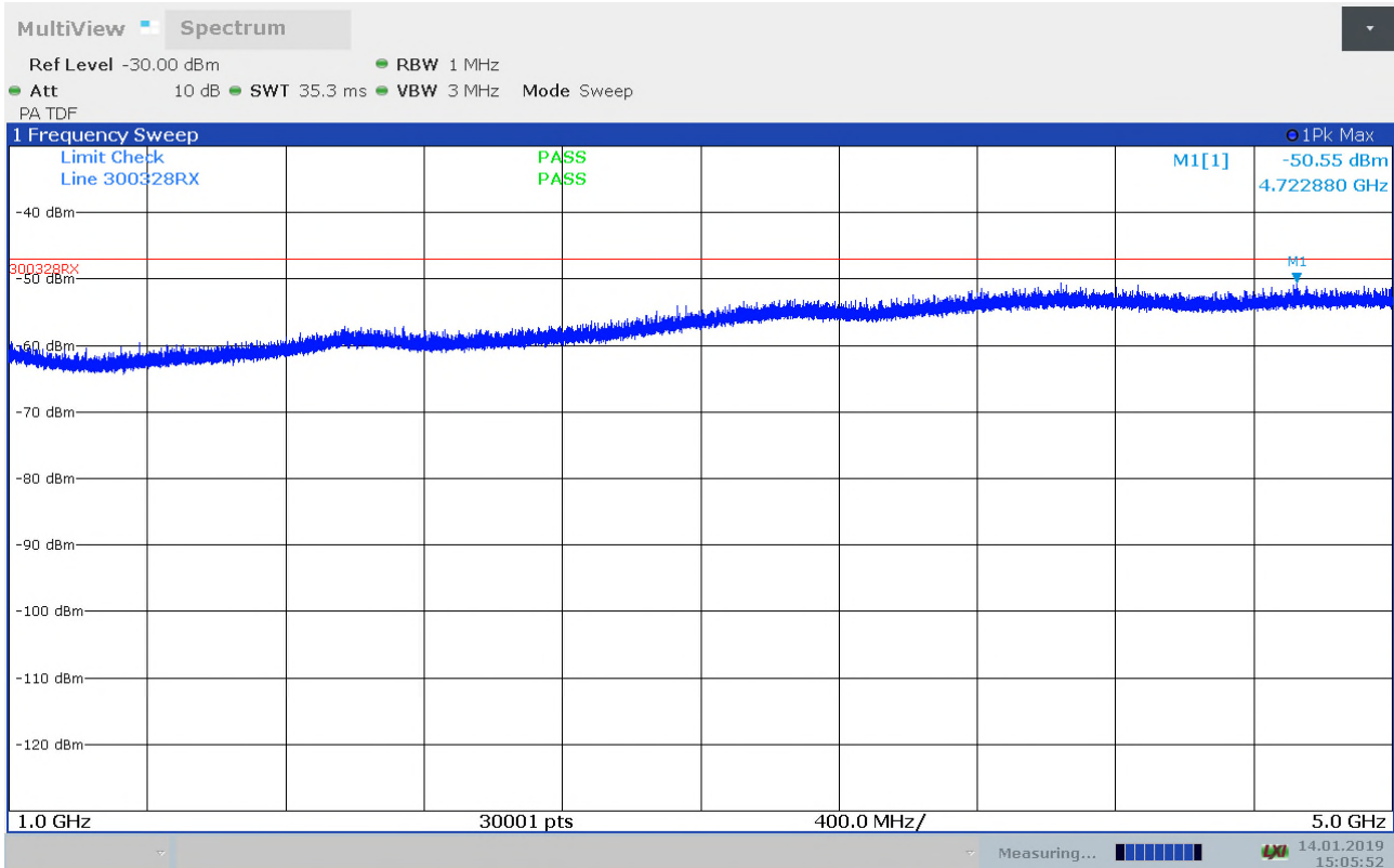
Receiver Emissions, radiated, 1 - 5GHz, ch2412MHz,HP
