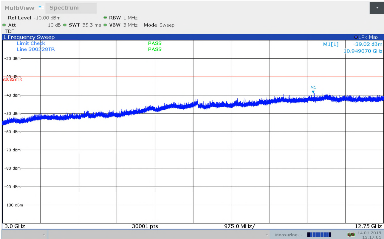
Radiated Emissions, 3 – 12.75GHz, 2412MHz, 11n, mcs0, HP
