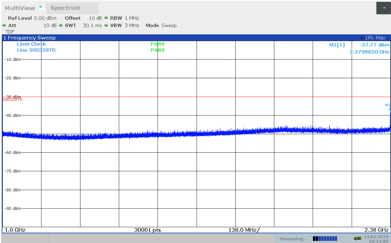
Radiated Emissions, 1 - 2.380GHz, 2412MHz,11g, 6Mbps, HP
