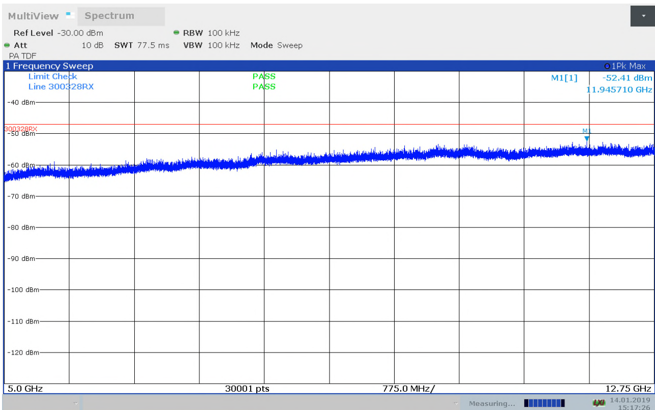
Receiver Emissions, radiated, 5 - 12.75GHz, ch2472MHz, VP, prescan
