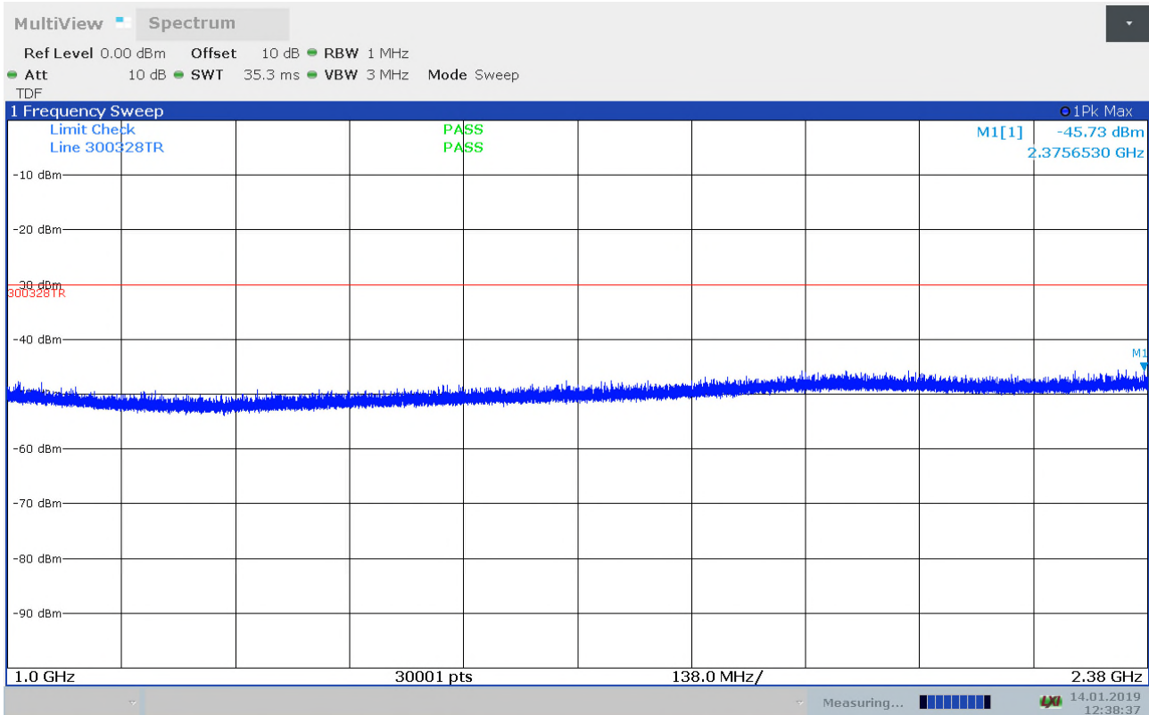
Radiated Emissions, 1 - 2.380GHz, 2472MHz,11g,6Mbps, HP
