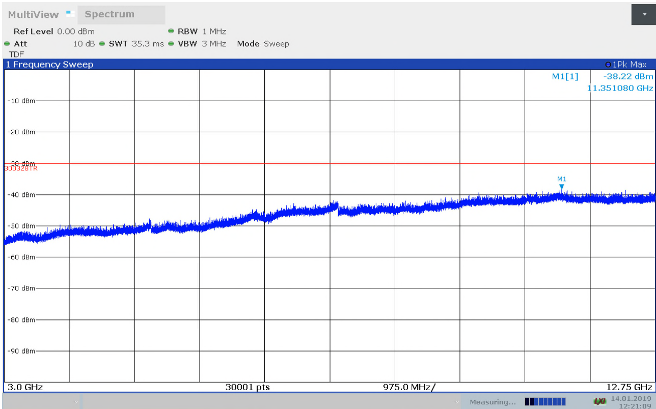
Radiated Emissions, 3 – 12.75GHz, 2412MHz, 11b, 6Mbps, HP
