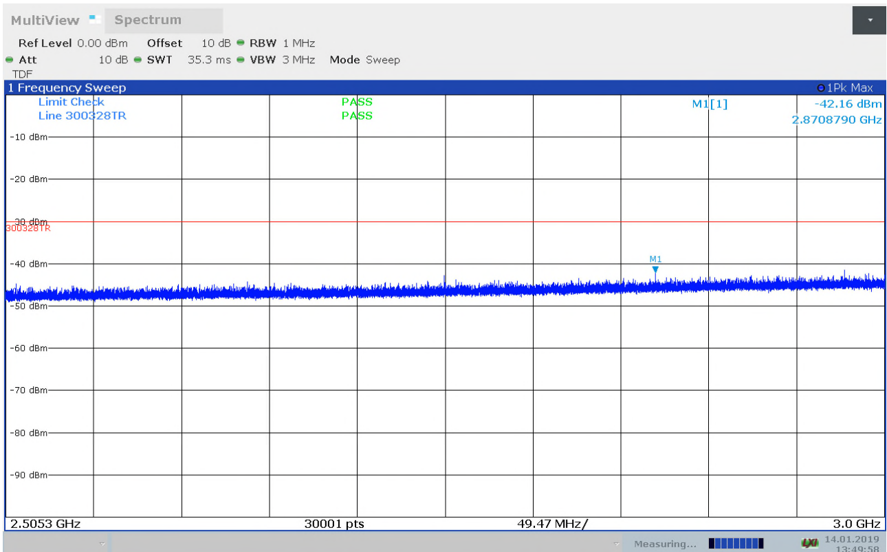
Radiated Emissions, 2.5035 - 3GHz, 2472MHz, 11n,mcs0,VP
