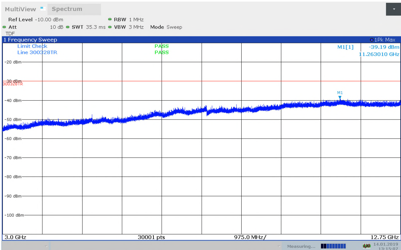
Radiated Emissions, 3 – 12.75GHz, 2412MHz, 11n, mcs0, VP
