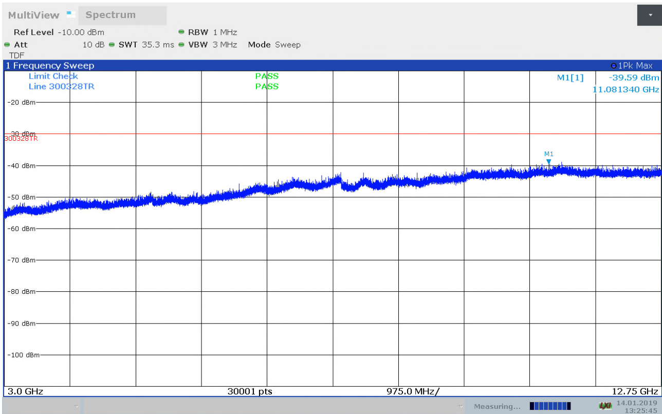
Radiated Emissions, 3 – 12.75GHz, 2472MHz, 11n, mcs0, VP
