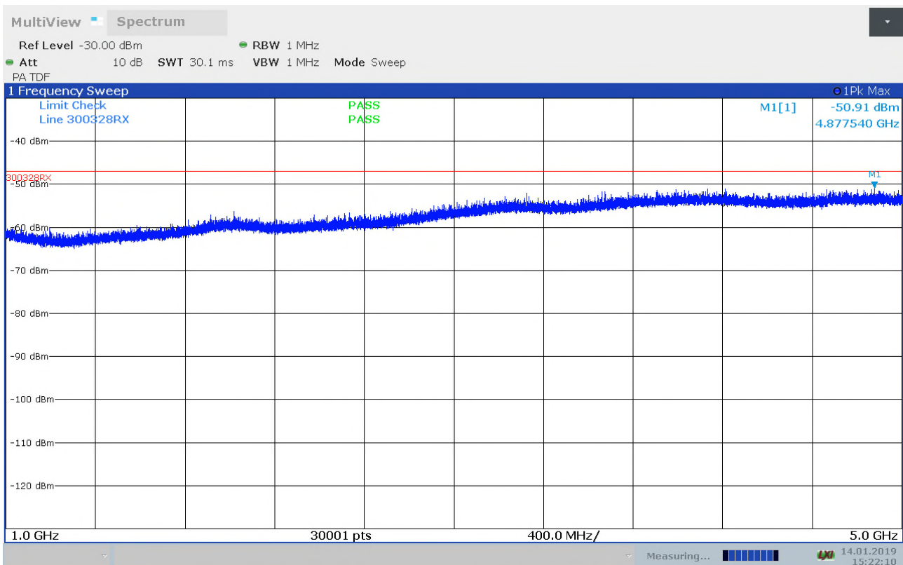
Receiver Emissions, radiated, 1 - 5GHz, ch2412MHz,VP
