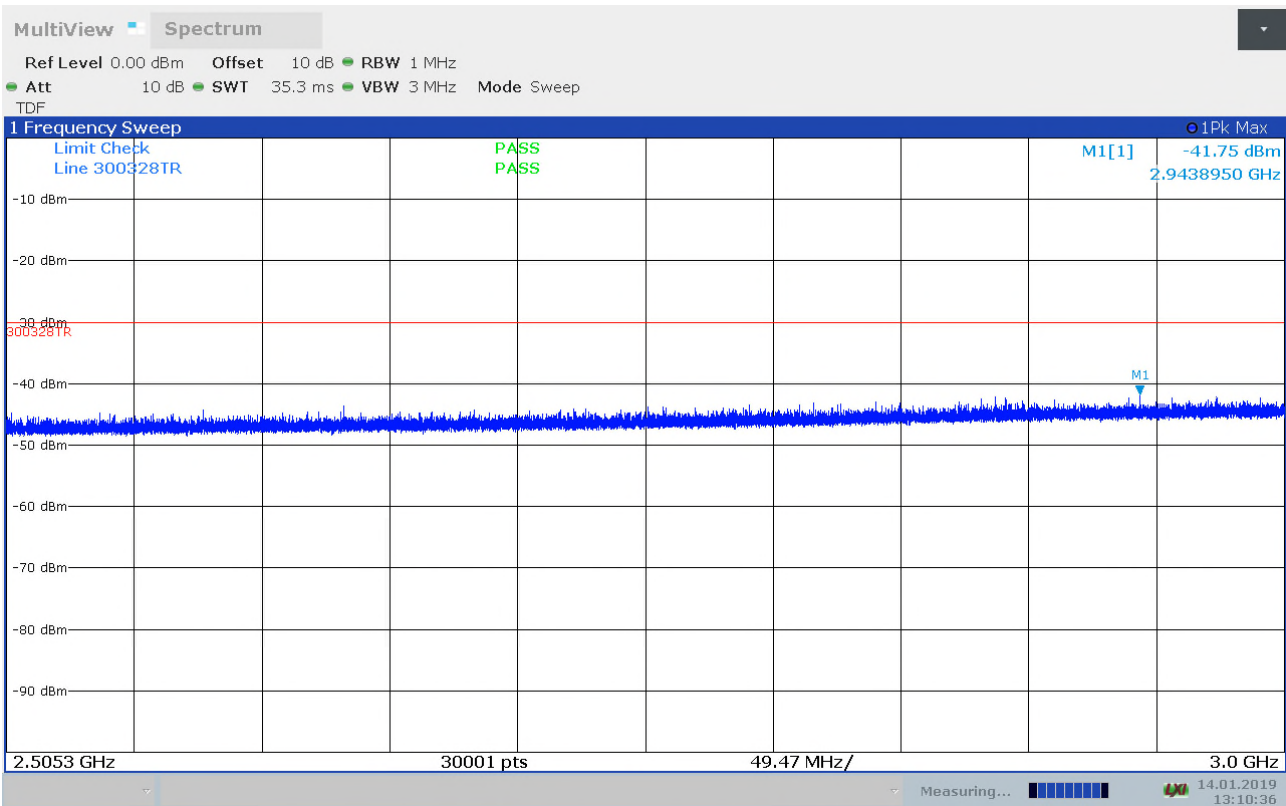
Radiated Emissions, 2.5035 - 3GHz, 2412MHz, 11n, mcs0, VP
