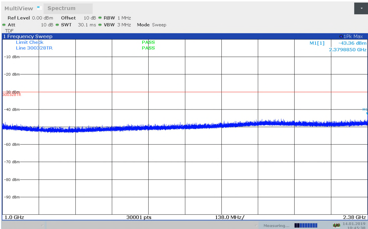
Radiated Emissions, 1 - 2.380GHz, 2412MHz, 11g, 6Mbps, VP
