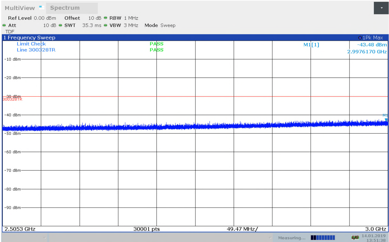
Radiated Emissions, 2.5035 - 3GHz, 2472MHz, 11n,mcs0, HP
