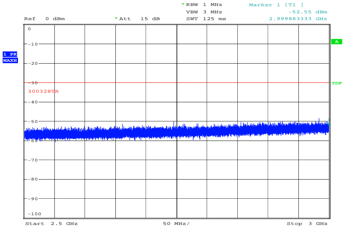
Radiated Emissions, 2.5035 - 3GHz, 2472MHz, 11g, 6Mbps, HP
