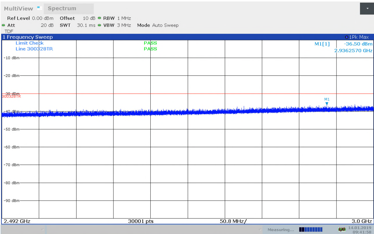
Radiated Emissions, 2.492 - 3GHz, 2412MHz,11b,1Mbps, VP
