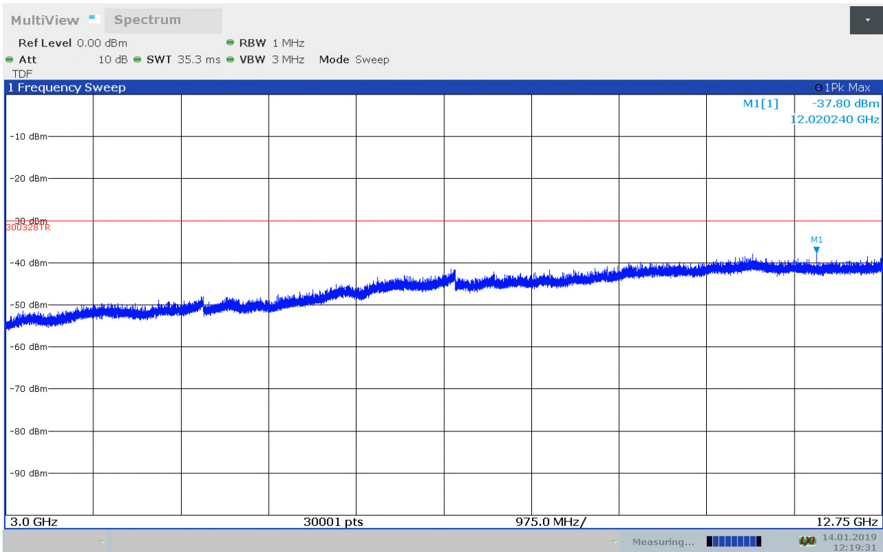
Radiated Emissions, 3 – 12.75GHz, 2412MHz, 11g, 6Mbps, VP
