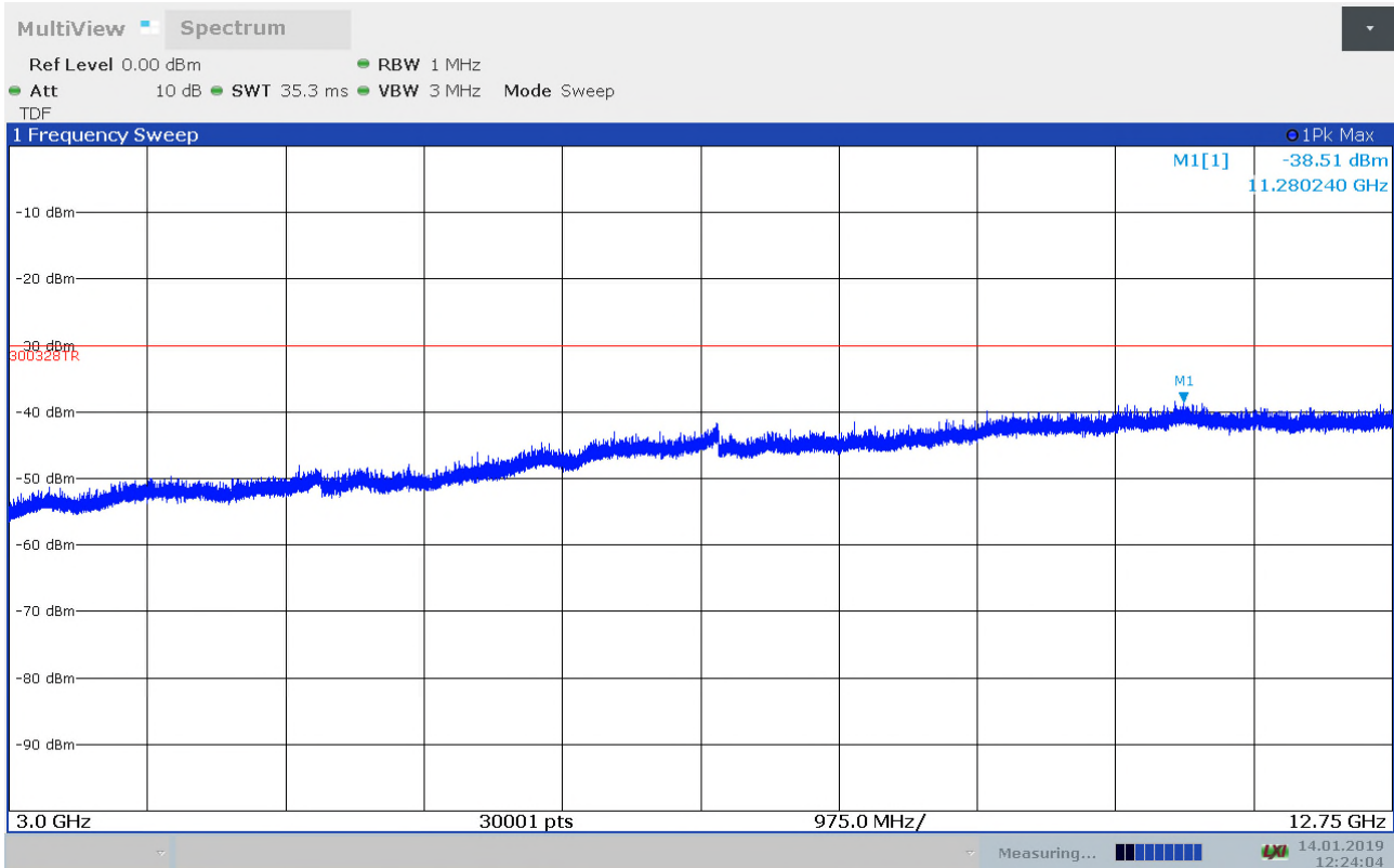
Radiated Emissions, 3 – 12.75GHz, 2472MHz, 11g,6Mbps, HP
