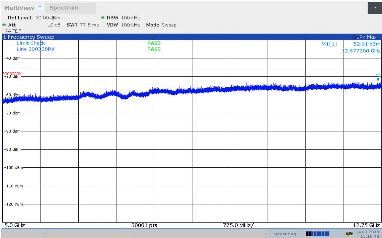
Receiver Emissions, radiated, 5 – 12.75GHz, ch2472MHz, HP, prescan
