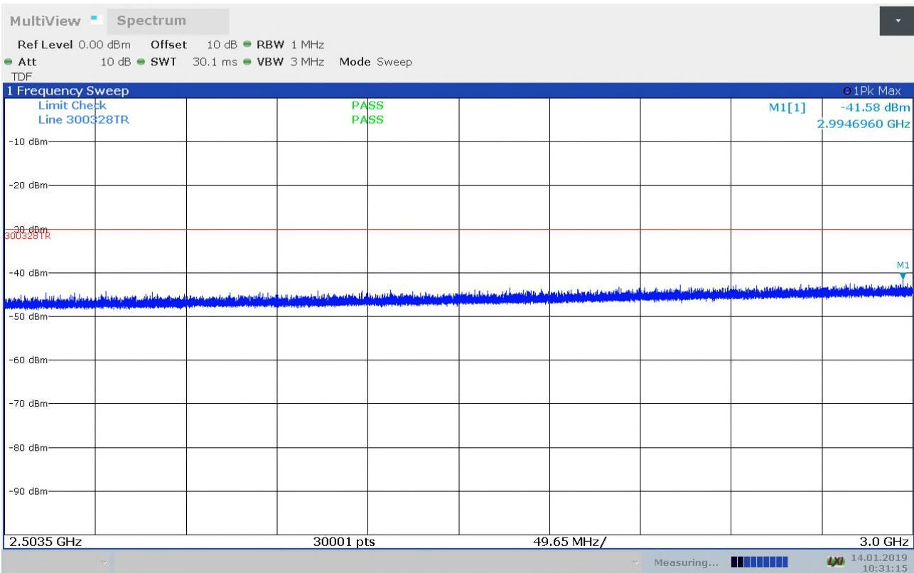
Radiated Emissions, 2.5035 - 3GHz, 2472MHz, 11b, 1Mbps, VP
