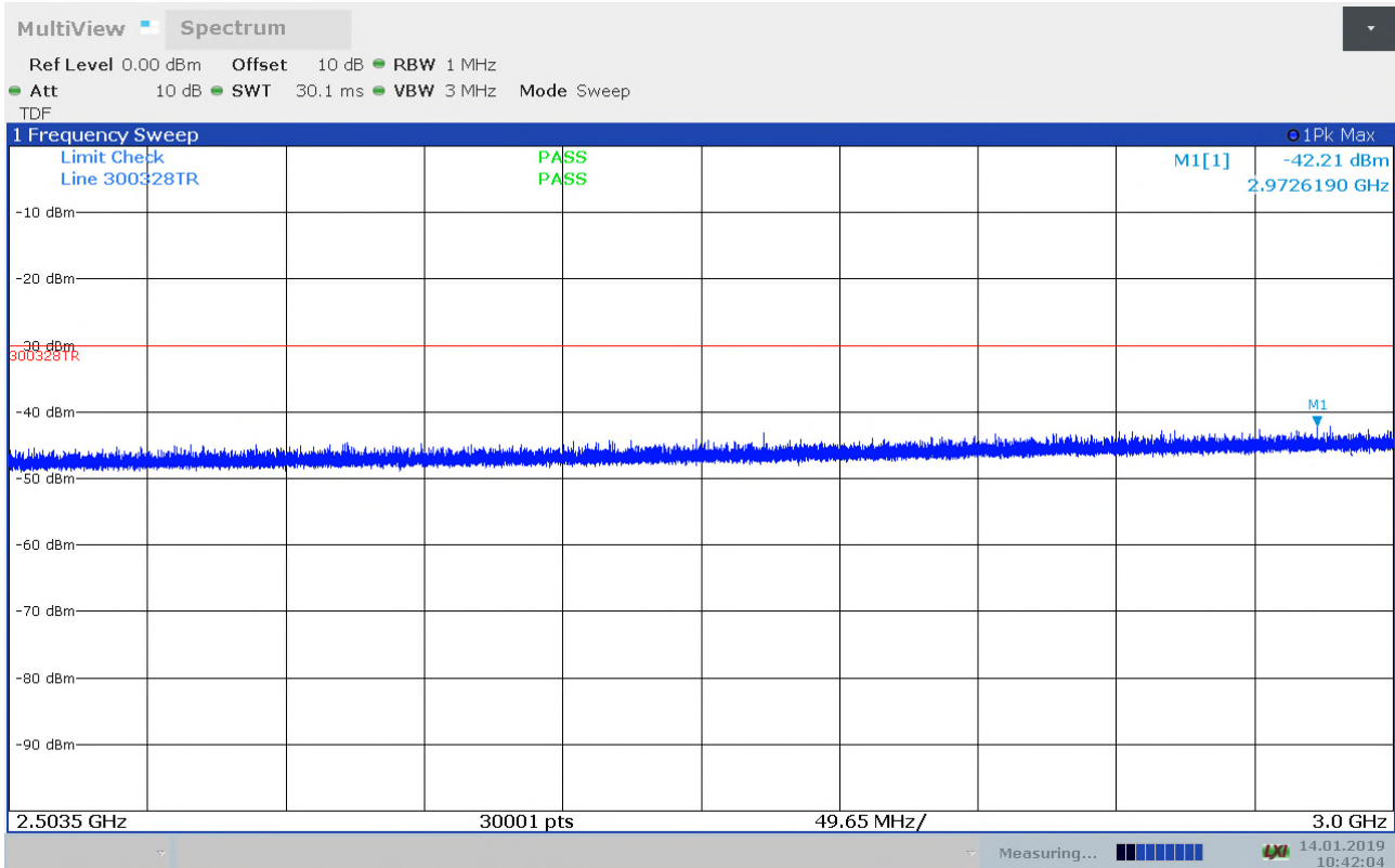
Radiated Emissions, 2.5035 - 3GHz, 2412MHz, 11g, 6Mbps, HP
