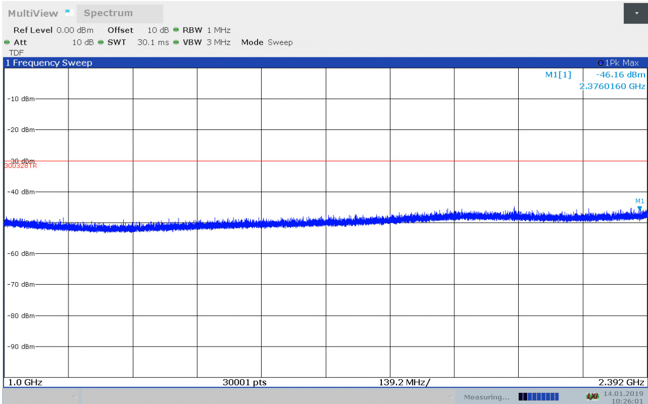
Radiated Emissions, 1 - 2.392GHz, 2472MHz,11b,1Mbps, HP
